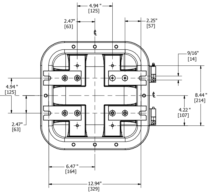
MOUNTING FEET
